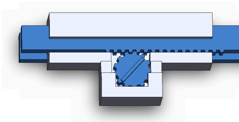
Figure 5. Rack & Pinion Assembly of E-Joint
