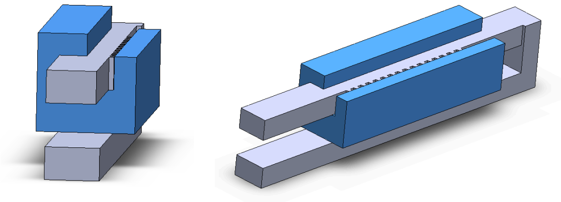
Figure 4. E-Joint Frame Around Sliding Rack
