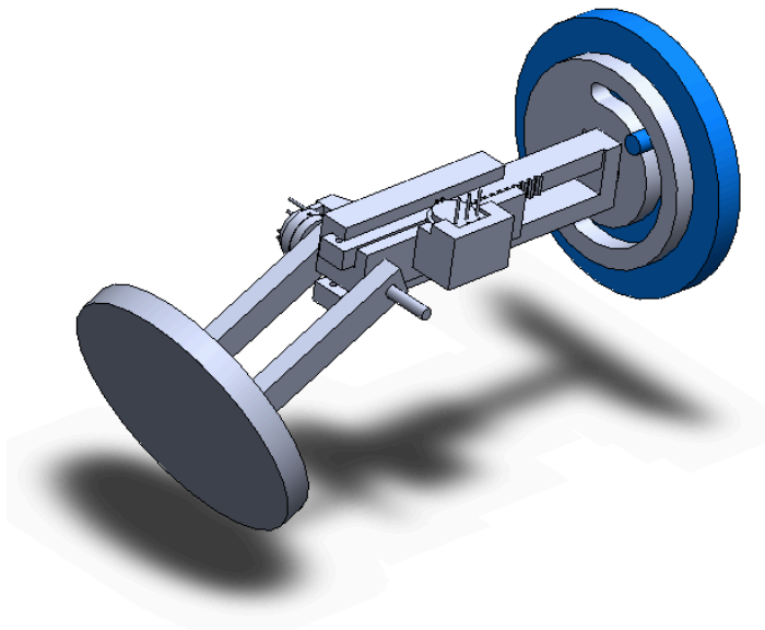
Figure 12. Final Rotational Joint in Assembly
