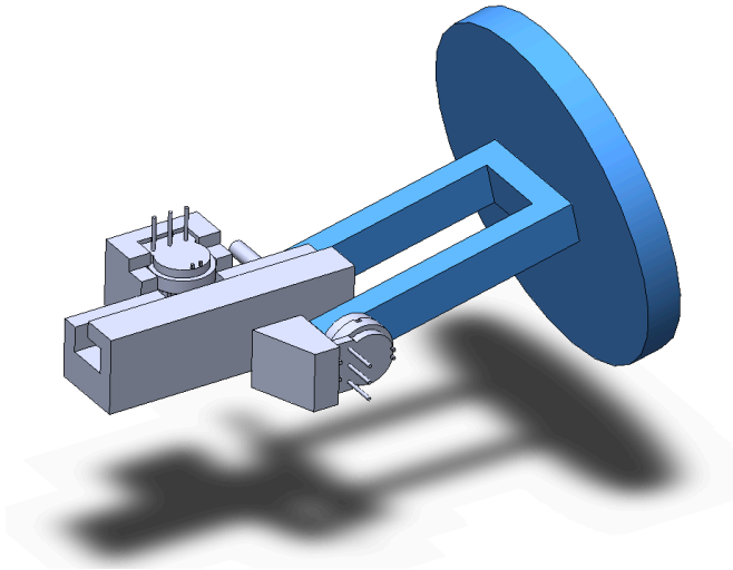
Figure 11. Final Bending Joint
