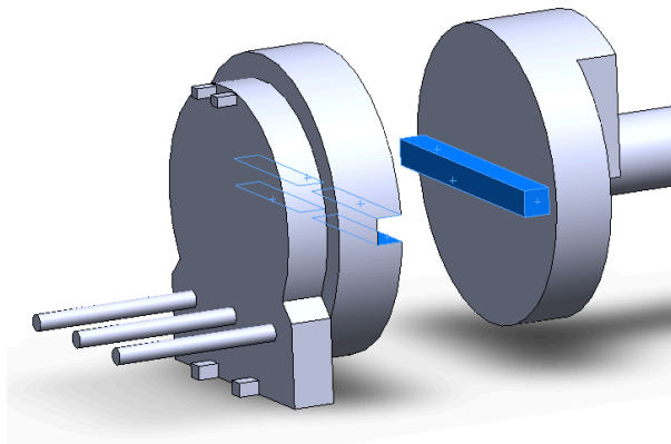
Figure 8. Pin / Potentiometer Mate
